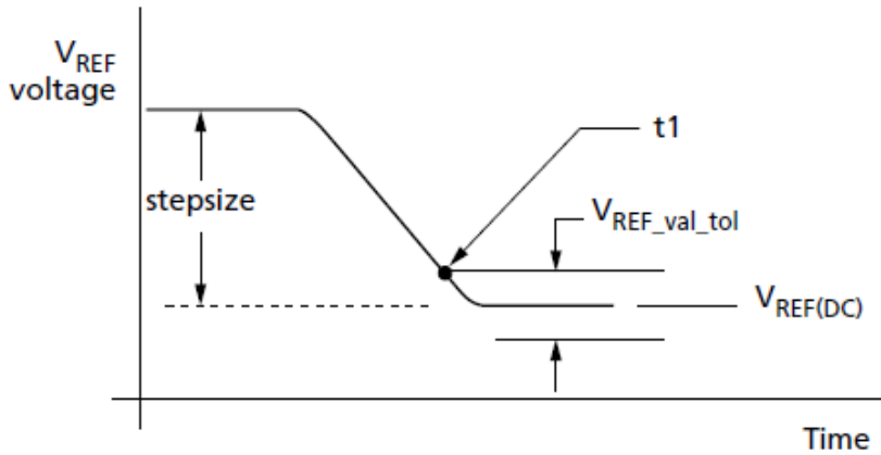
V_{REF(DQ)} Single-Step Size Decrement
