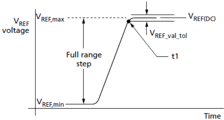
V_{REF(DQ)} Full Step from V_{REF,min} to V_{REF,max}
