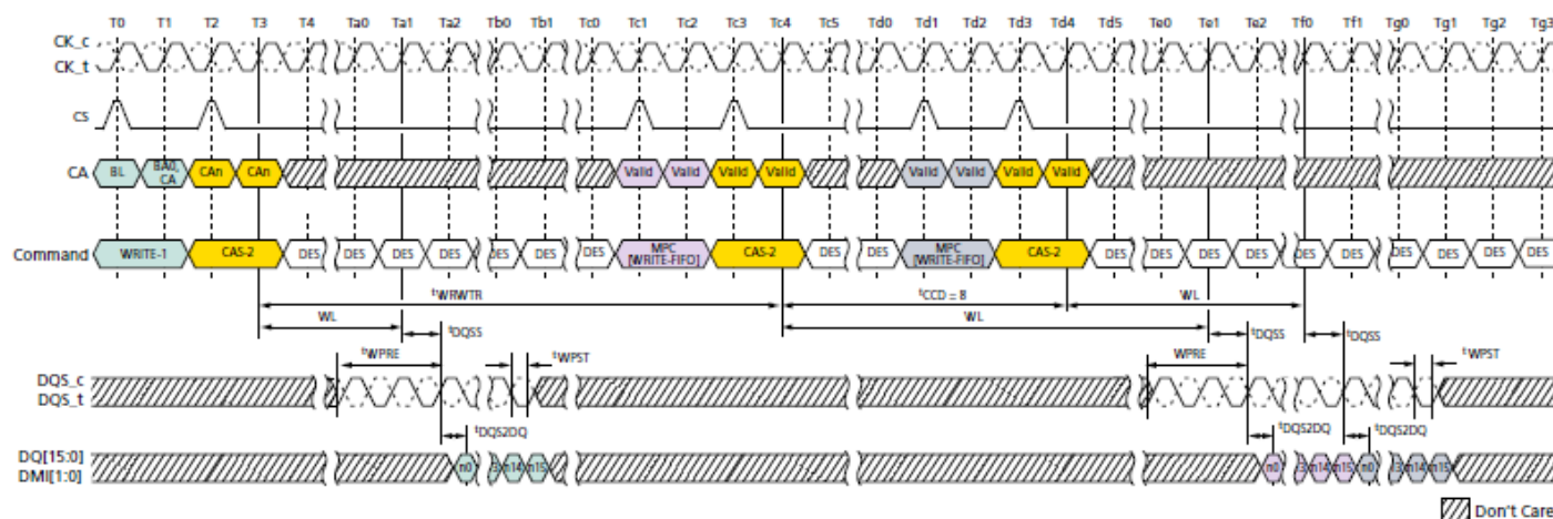
WRITE-to-MPC[WRITE-FIFO] Operation Timing
