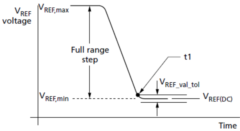
V REF(CA) Full Step from V REF,max to V REF,min
