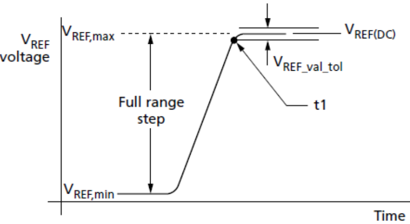
V REF(CA) Full Step from V REF,min to V REF,max
